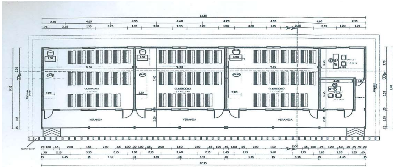
PLAN DE DISTRIBUTION DISTRIBUTION PLAN
